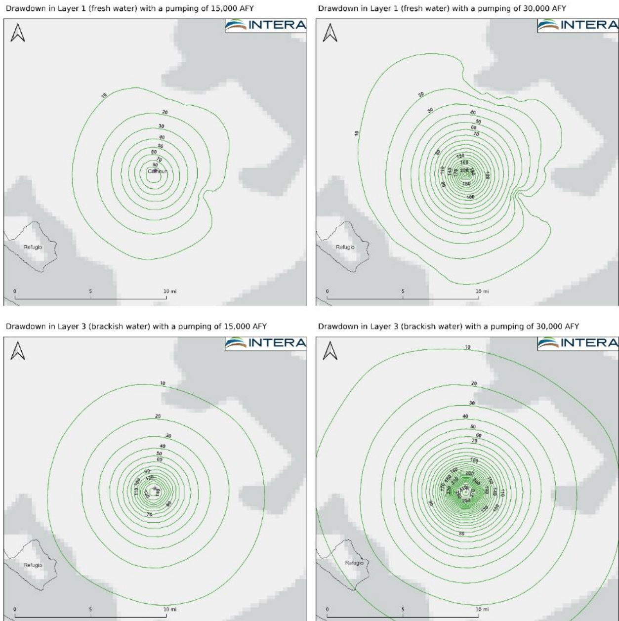
Figure B-5. Simulated drawdowns after 30-year pumping at well field #2 at a rate of 15,000 AFY (left) and 30,000 AFY (right). RCH is used for cells at land surface to represent recharge. GHB is used for cells at land surface to represent discharge.
