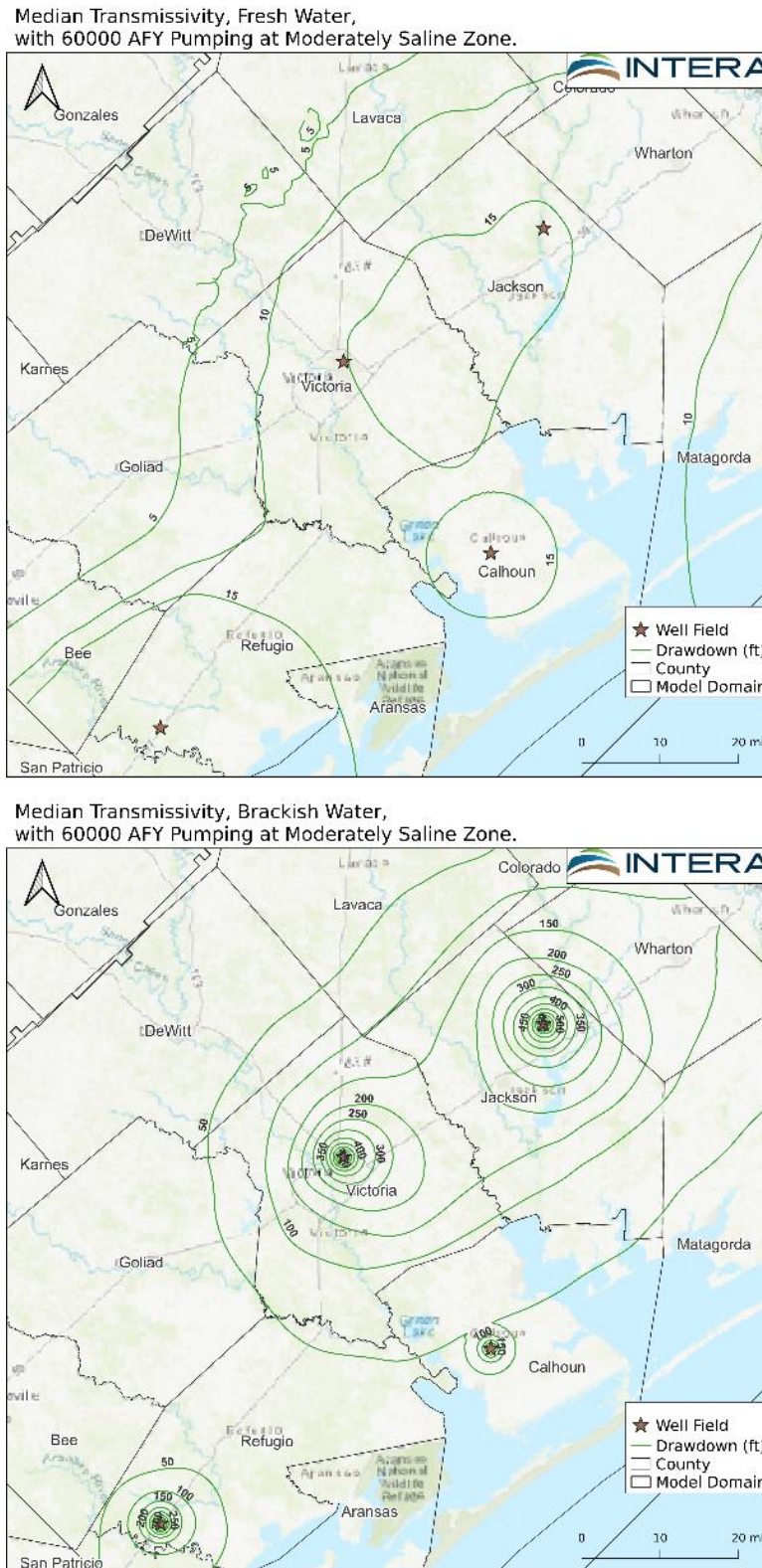
Figure 2-22. Simulated drawdown in freshwater zone (top) and brackish water zone (bottom) due to four well fields at sites of median transmissivity in the moderately saline zone.
