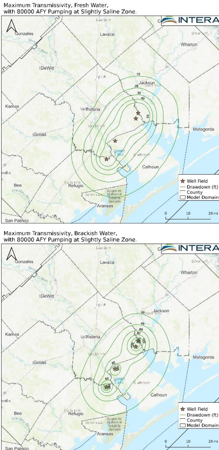
Figure 2-19. Simulated drawdown in freshwater zone (top) and brackish water zone (bottom) due to four well fields at sites of maximum transmissivity in the slightly saline zone.
