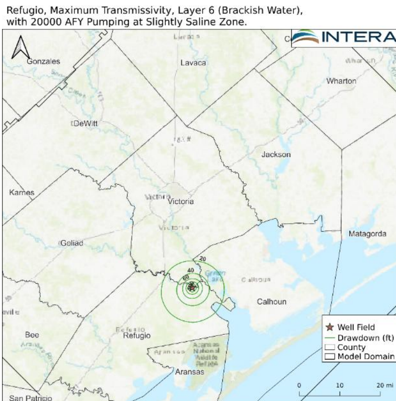
Figure 2-5. Simulated drawdown in freshwater zone (top) and brackish water zone (bottom) due to well field #3.
