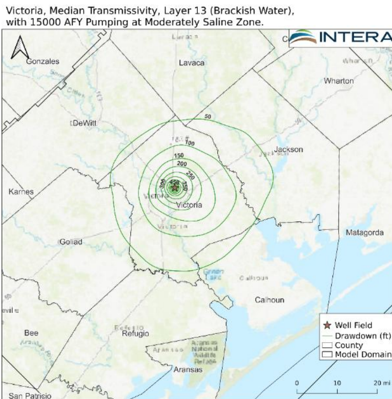
Figure 2-18. Simulated drawdown in freshwater zone (top) and brackish water zone (bottom) due to well field #16. The drawdown in freshwater zone is less than 2 ft.
